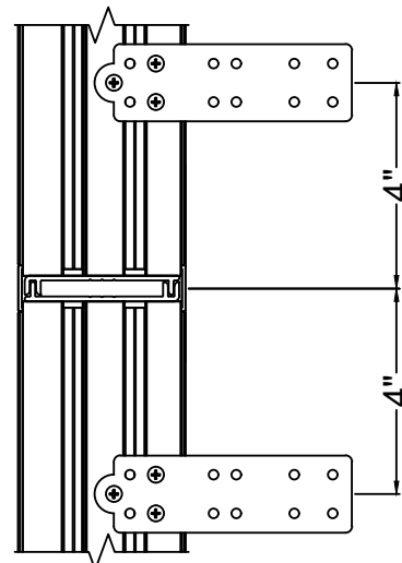
STRAP ANCHOR DETAIL AT HORIZONTAL MULL
