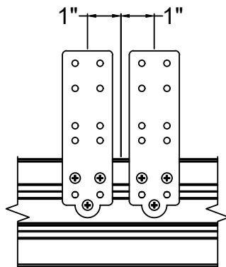
STRAP ANCHOR DETAIL AT VERTICAL MULLION
